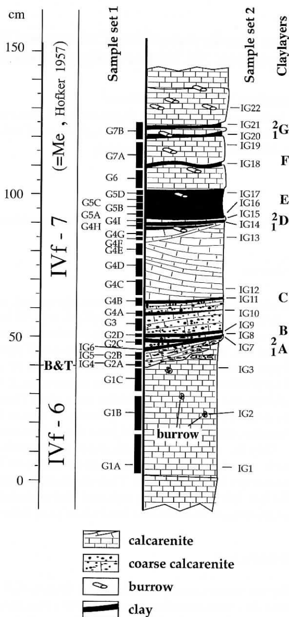
Figure 2. Lithologic column of the main K/T section as exposed in the Geulhemmerberg caves. B&T = Berg en Terblijt Horizon. Lithologic subdivision after Felder (1975) and Felder and Bosch (in press).
