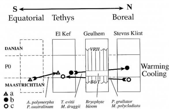
Figure 5. Schematic illustration of the dinoflagellate (cyst) migrations at K/T times. a) Tropical, b) Tethyan, c) Boreal species.
