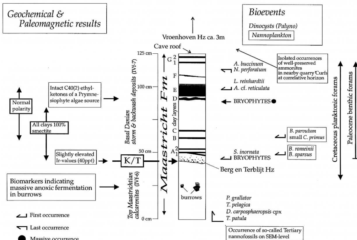
Figure 3. Overview of the principal results of the Geulhemmerberg Deep Dark Hole Project as reported in this issue. The K/T boundary is drawn at the Berg en Terblijt Horizon.
