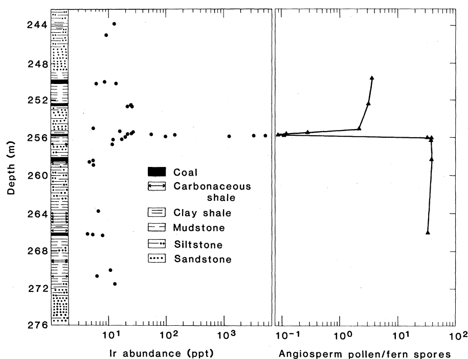
Fig. 1. Iridium abundances (circles) and ratios of angiosperm pollen to fern spores (triangles) as a function of core depth and lithology. The plotted Ir abundances in parts per trillion (parts per 10^{12} ) are derived from radiochemically separated samples. The curve through the pollen data is drawn to guide the eye.
