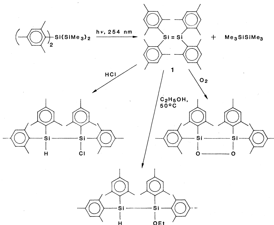
Fig. 1. Proposed scheme for the synthesis of tetramesityldisilene (1) and for the reaction of 1 with HCl, ethanol, and \text{O}_2 ; Me, methyl; Et, ethyl.
