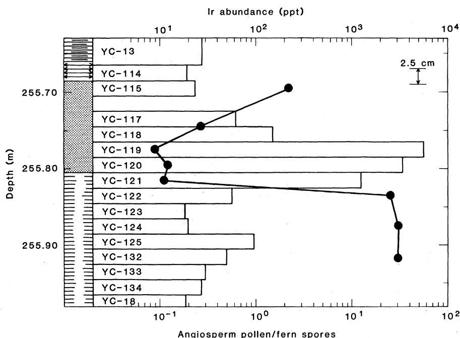
Fig. 2. Expanded view of the data of Fig. 1 in the vicinity of the Ir anomaly and the pollen break. The Ir abundances are given by the histogram and the angiosperm pollen/fern spore ratios by the circles. The curve is drawn to guide the eye. The lithologic symbols are the same as in Fig. 1 except for coal, which is shown by stipple.
