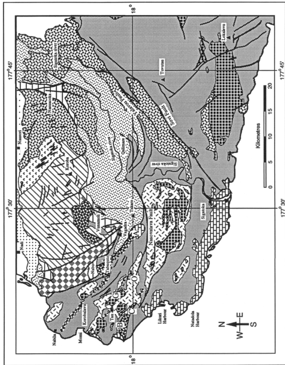
Figure 2.4: Geological map of SW Viti Levu based on Hathway and Colley (1989) and Rodda and Band (1966).
