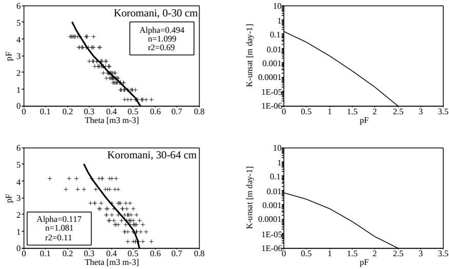
Figure 4.7: Soil moisture retention curves and modelled unsaturated hydraulic conductivities versus pF for the top- ( n = 13 ) and subsoil ( n = 7 ) of the Koromani forest plot.
