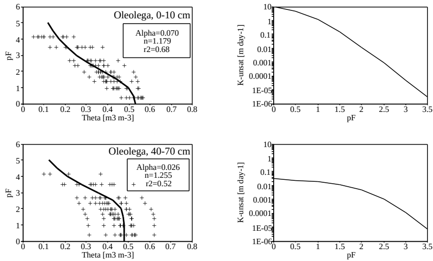
Figure 4.8: Soil moisture retention curves and modelled unsaturated hydraulic conductivities versus pF for the top- ( n = 11 ) and subsoil ( n = 11 ) in the Oleolega catchment.
