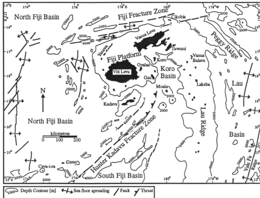
Figure 2.3: Present regional tectonic setting of the Fiji archipelago (after Rodda, 1989).
