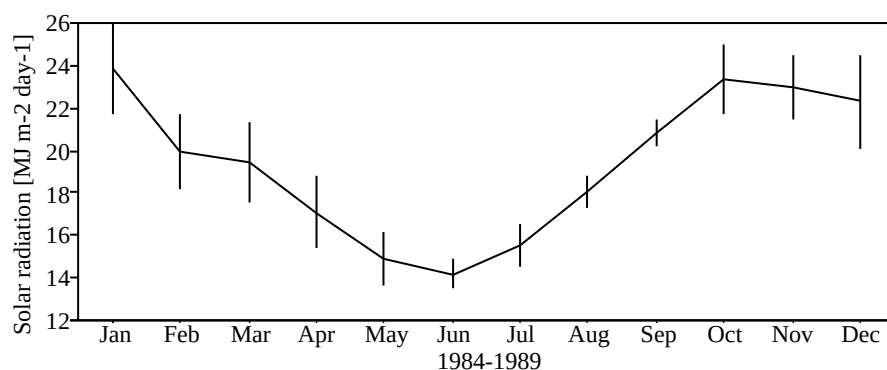
Figure 2.13: Monthly averages and standard deviations of solar radiation ( R_s \downarrow , in \text{MJ m}^{-2} \text{ day}^{-1} ) as measured at Nadi Airport (1984–1989; source: Fiji Meteorological Service, Nadi).
